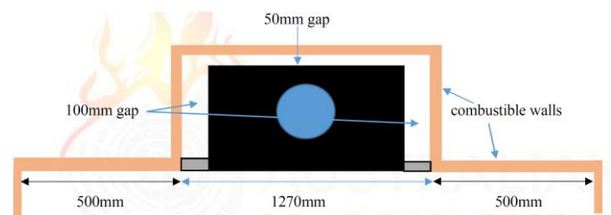
Figure No.18 - Top view of safety distances of Loire 1000 inbuild and zero clearance box
