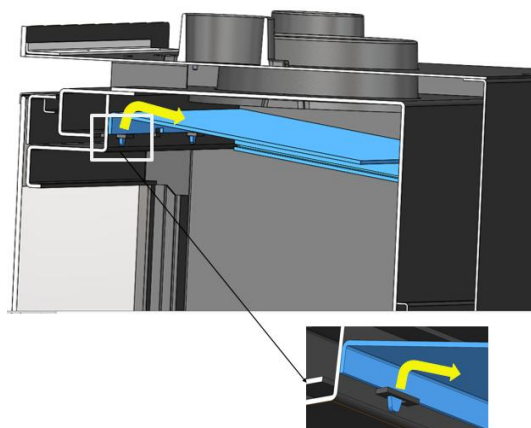
Figure No.38 - Dismantling the LOIRE steel deflector
