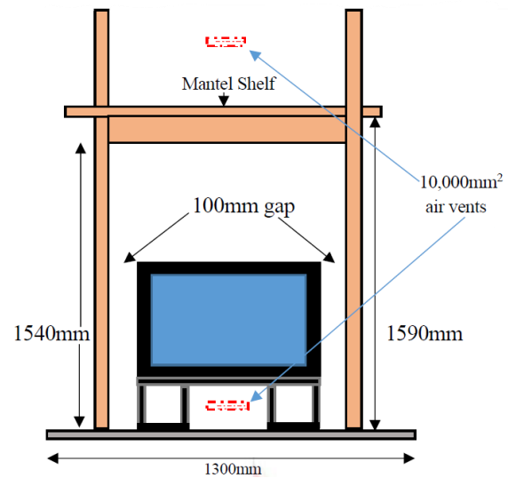
Figure No.16 - Front view of safety distances of Loire 1000 inbuild and zero clearance box
