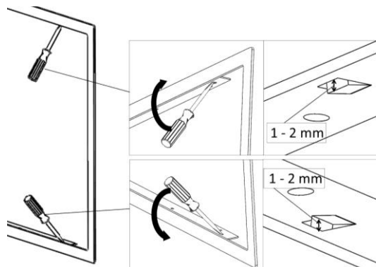
Figure No.28 - Bending the tabs
