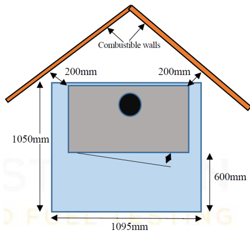
Figure No.8 - Safety distances of Loire 800 in corner position
