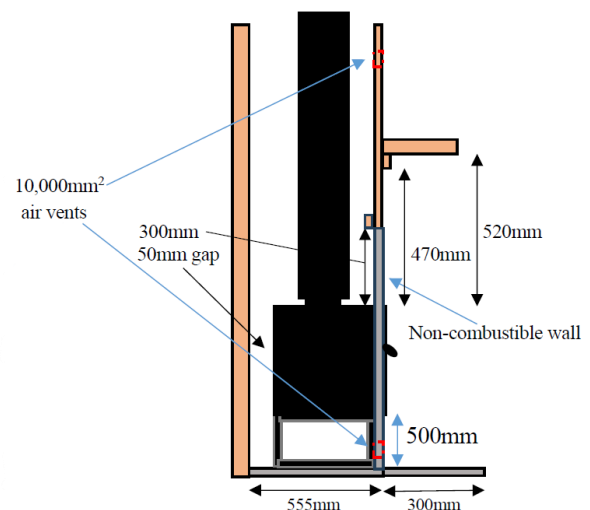
Figure No.17 - Profile view of safety distances of Loire 800 and Loire 1000 inbuild and zero clearance box
