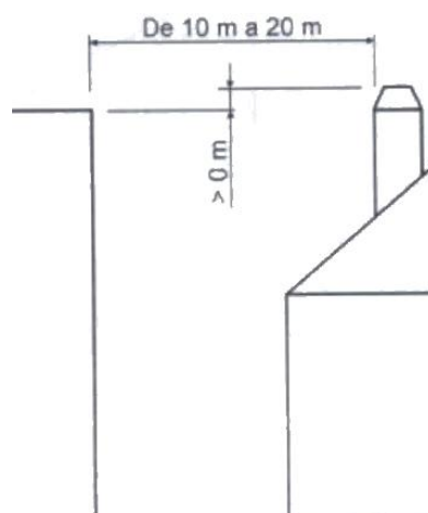
Figure No.33 - Distances between the chimney crown and objects within a radius of between 10 and 20m
