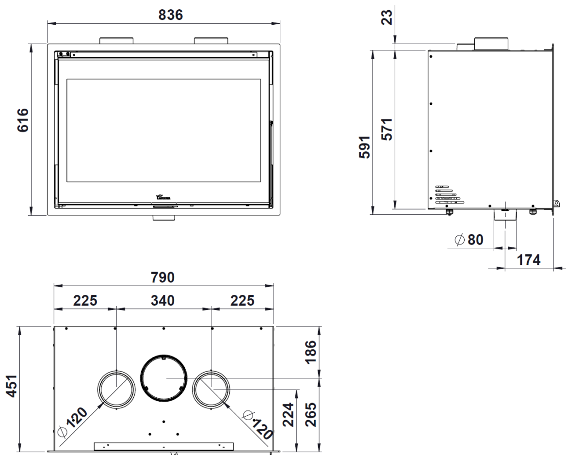
Figure No.1 - Dimensions of the LOIRE 800 In Built appliance in mm
