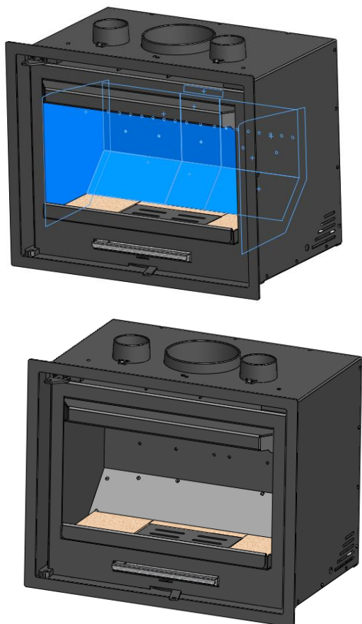
Figure No.37 - Dismantling the LOIRE vermiculite deflector
